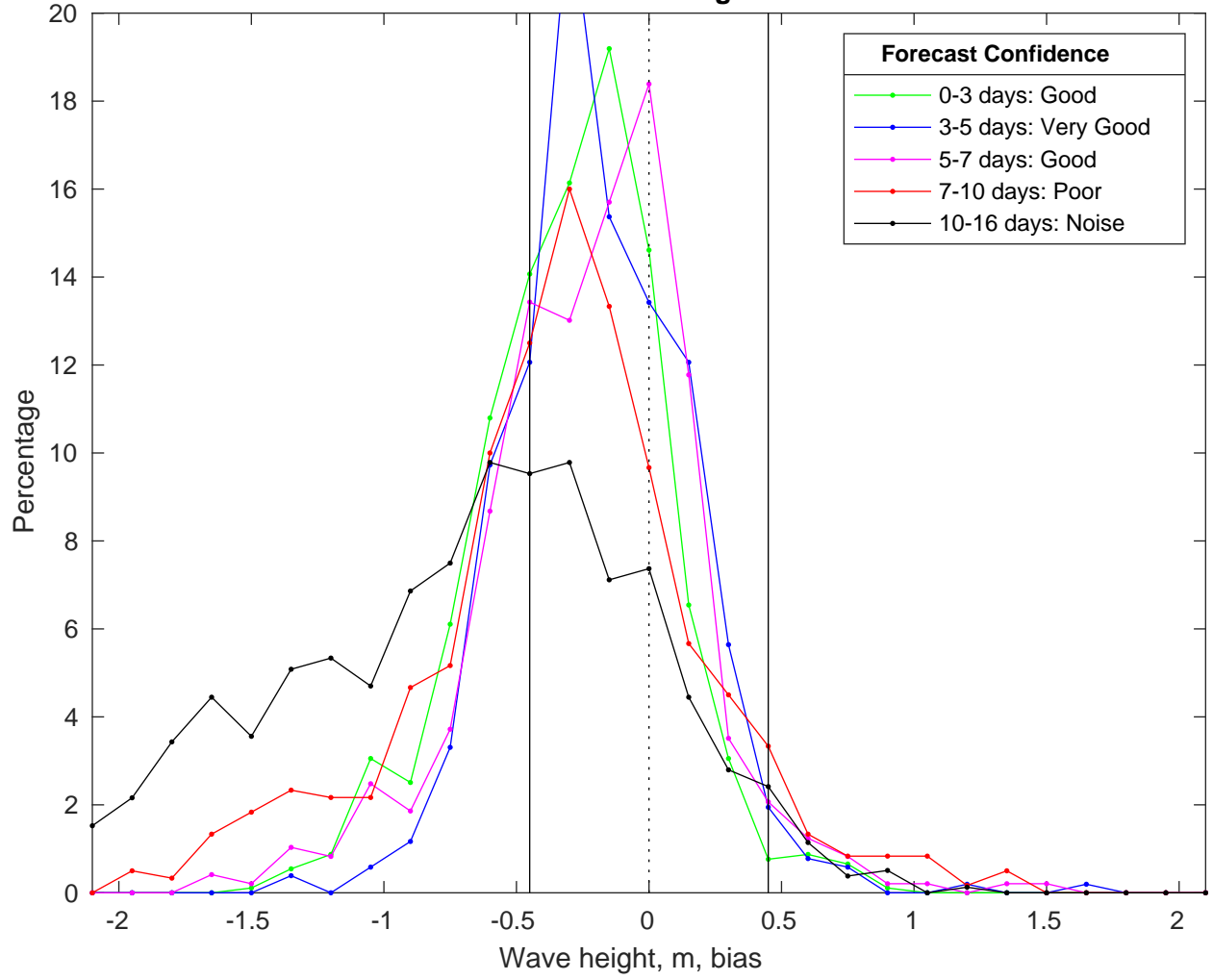
NDBC 46028 vs GFSWaves Bias Histogram: 15-Jan-2025
