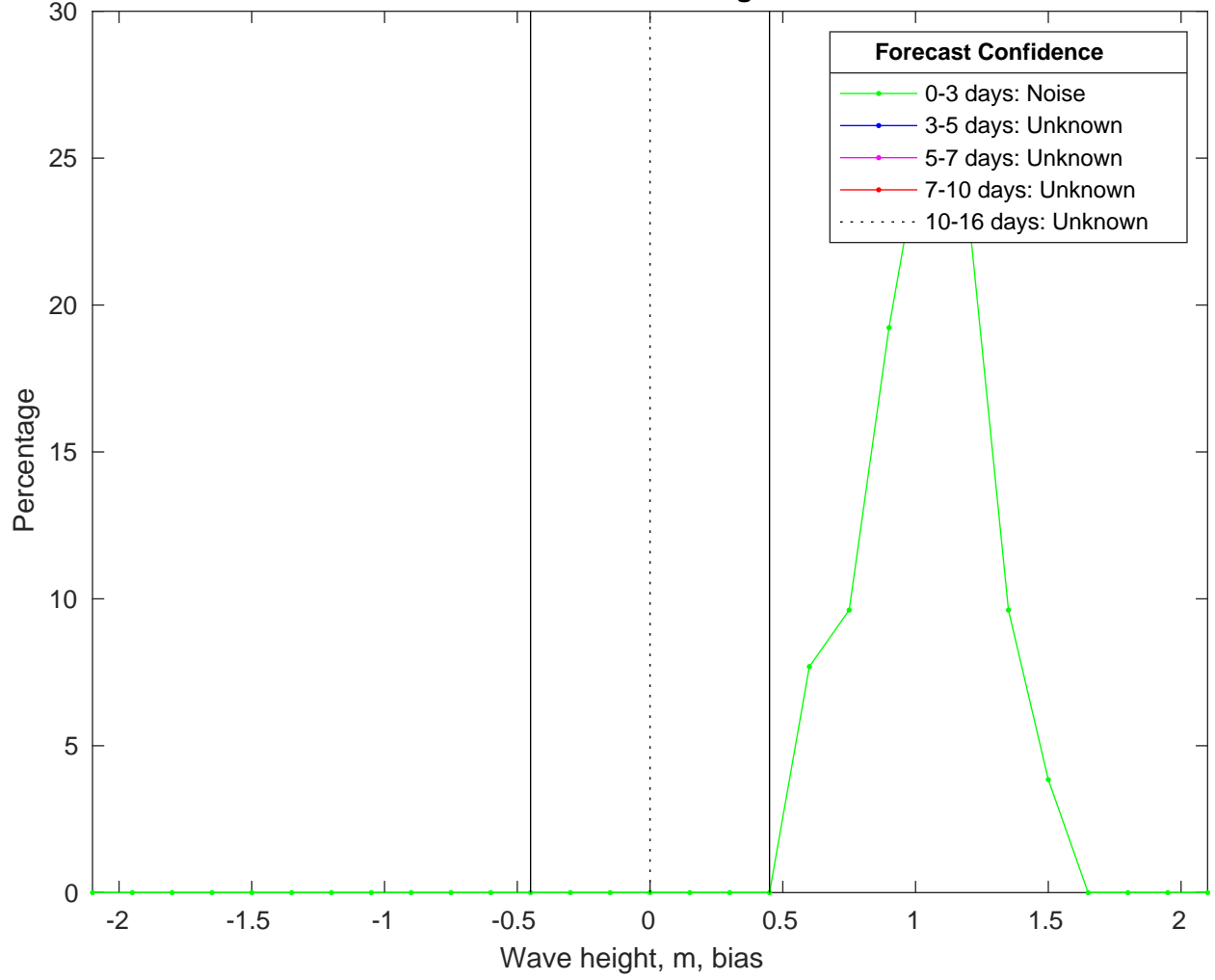
NDBC 46053 vs CMEMSWaves Bias Histogram: 15-Jan-2025
