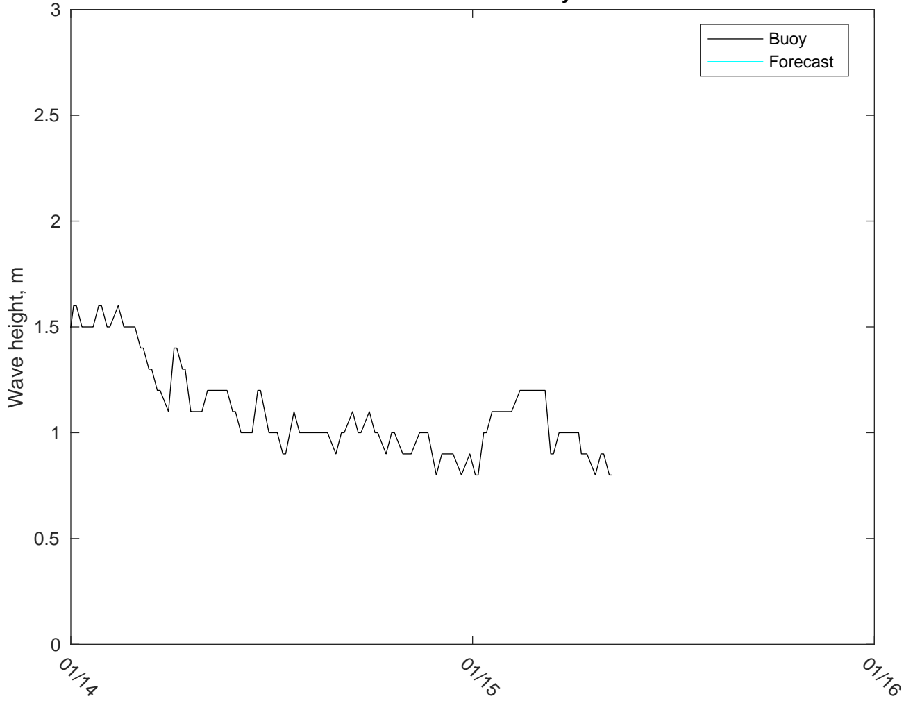
NDBC 46053 vs GFSWaves: 5 to 7 day forecast
