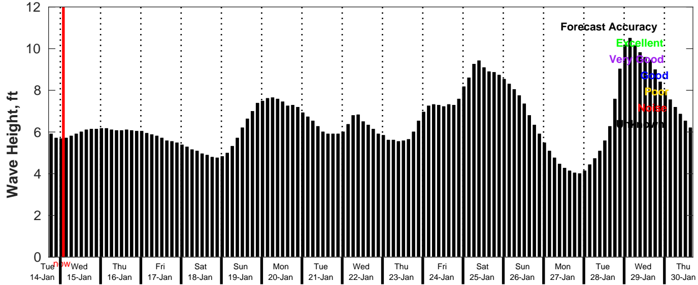
GFS Wave Forecast for NDBC 46053 from 14-Jan-2025 17:00:00 to 30-Jan-2025 17:00:00
