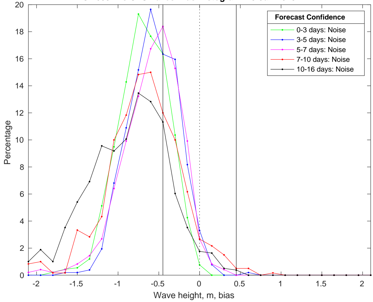
NDBC 46054 vs GFSWaves Bias Histogram: 15-Jan-2025
