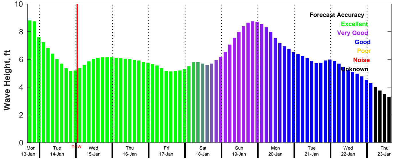
CMEMS Wave Forecast for NDBC 46054 from 13-Jan-2025 16:00:00 to 23-Jan-2025 16:00:00
