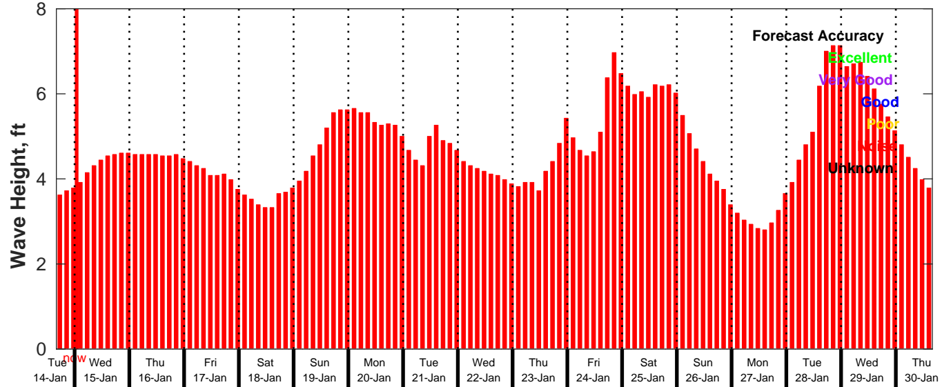
GFS Wave Forecast for NDBC 46054 from 14-Jan-2025 16:00:00 to 30-Jan-2025 16:00:00
