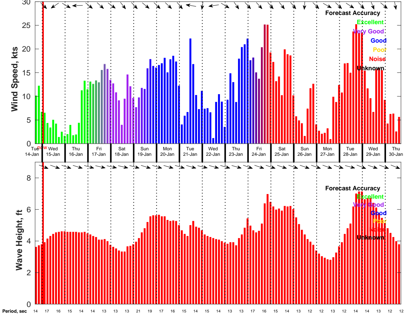
Wind & Wave Forecast for NDBC 46054 from 14-Jan-2025 16:00:00 to 30-Jan-2025 16:00:00
