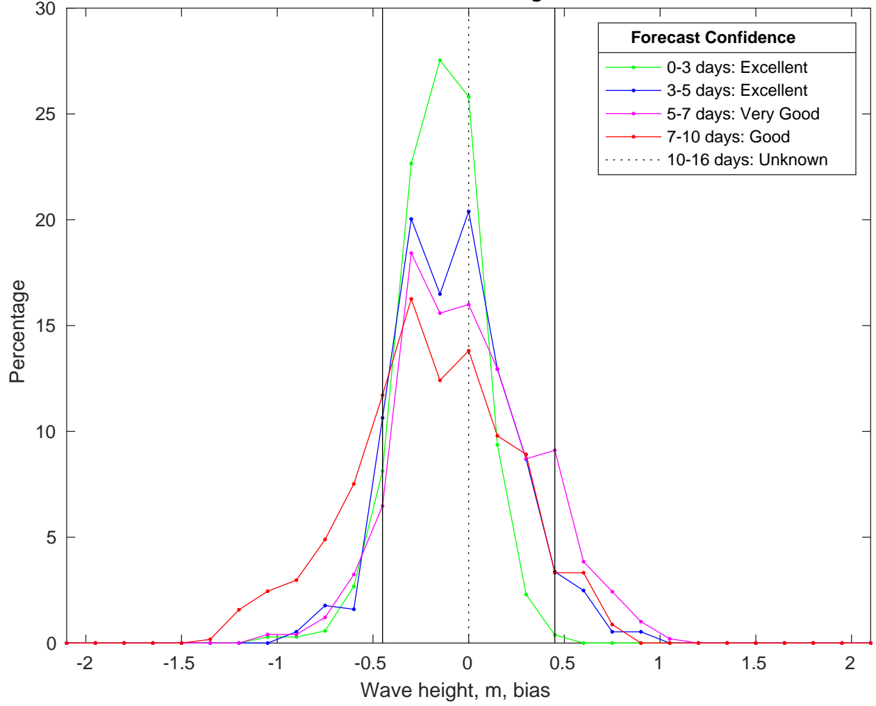
NDBC 46069 vs CMEMSWaves Bias Histogram: 15-Jan-2025
