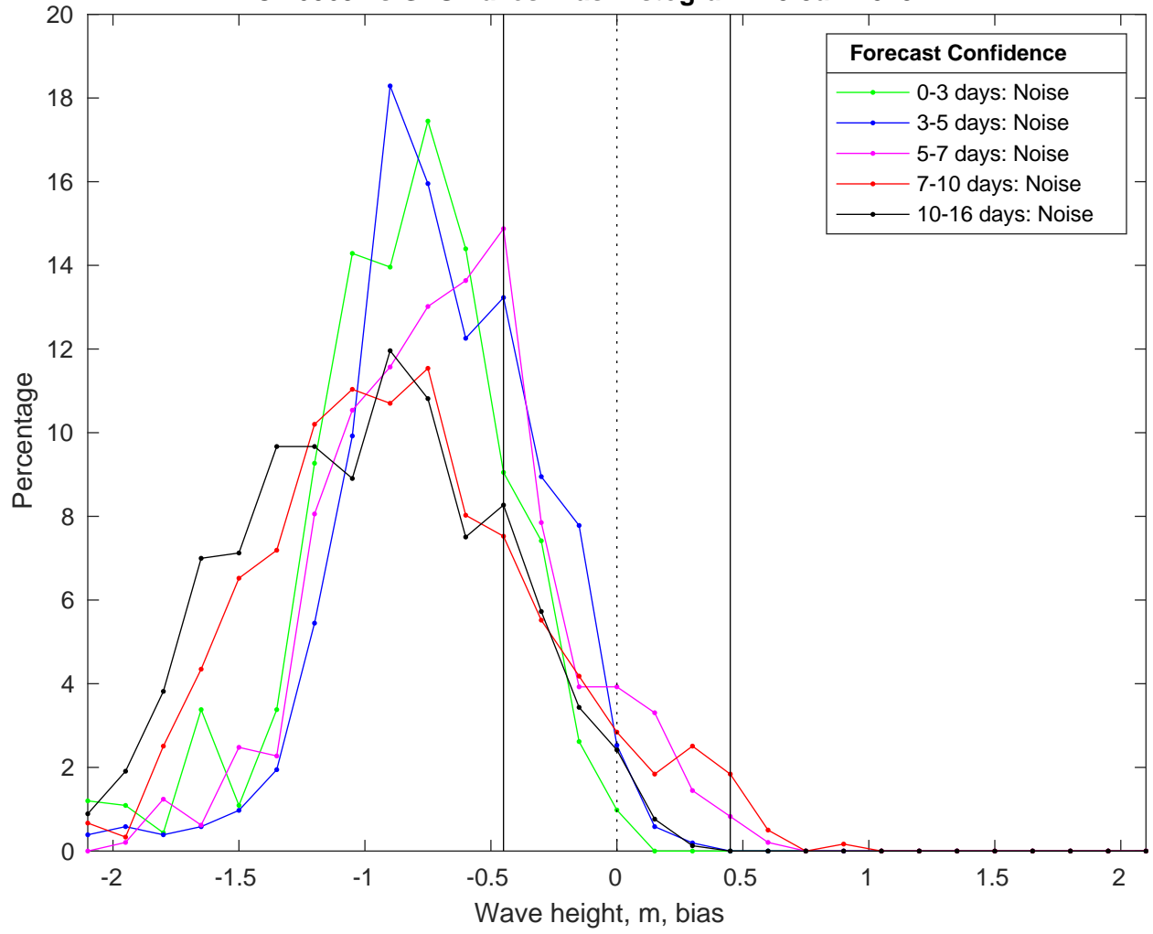
NDBC 46069 vs GFSWaves Bias Histogram: 15-Jan-2025
