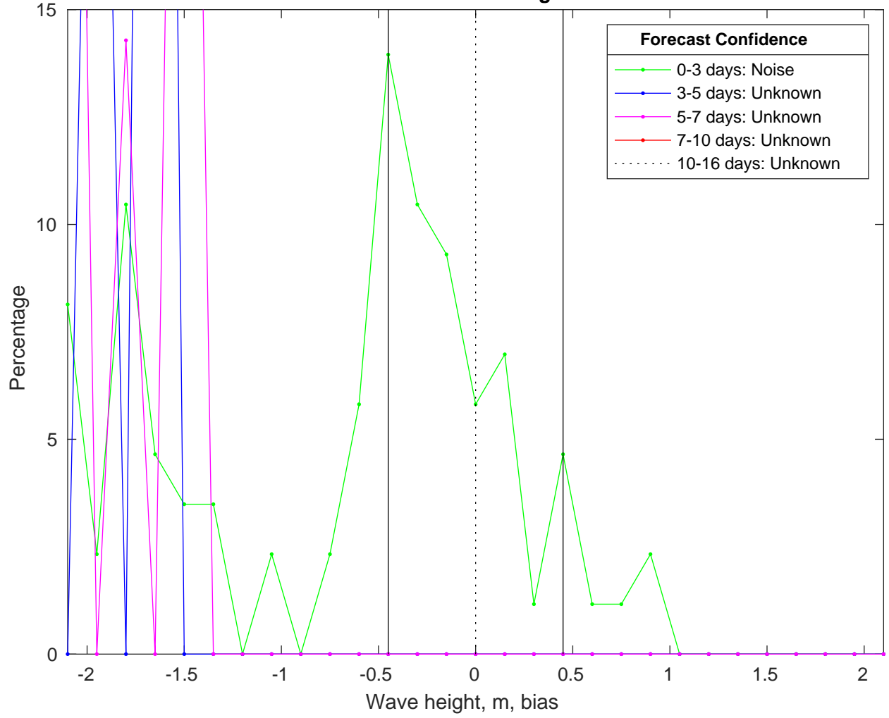
NDBC 46246 vs CMEMSWaves Bias Histogram: 15-Jan-2025
