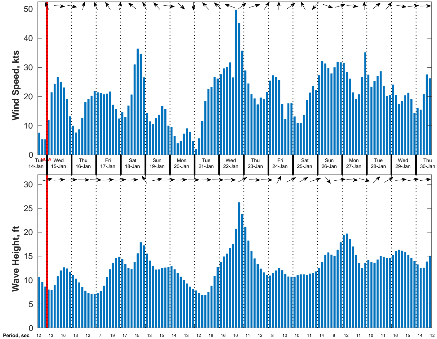
Wind & Wave Forecast for NDBC 46246 from 14-Jan-2025 15:00:00 to 30-Jan-2025 15:00:00
