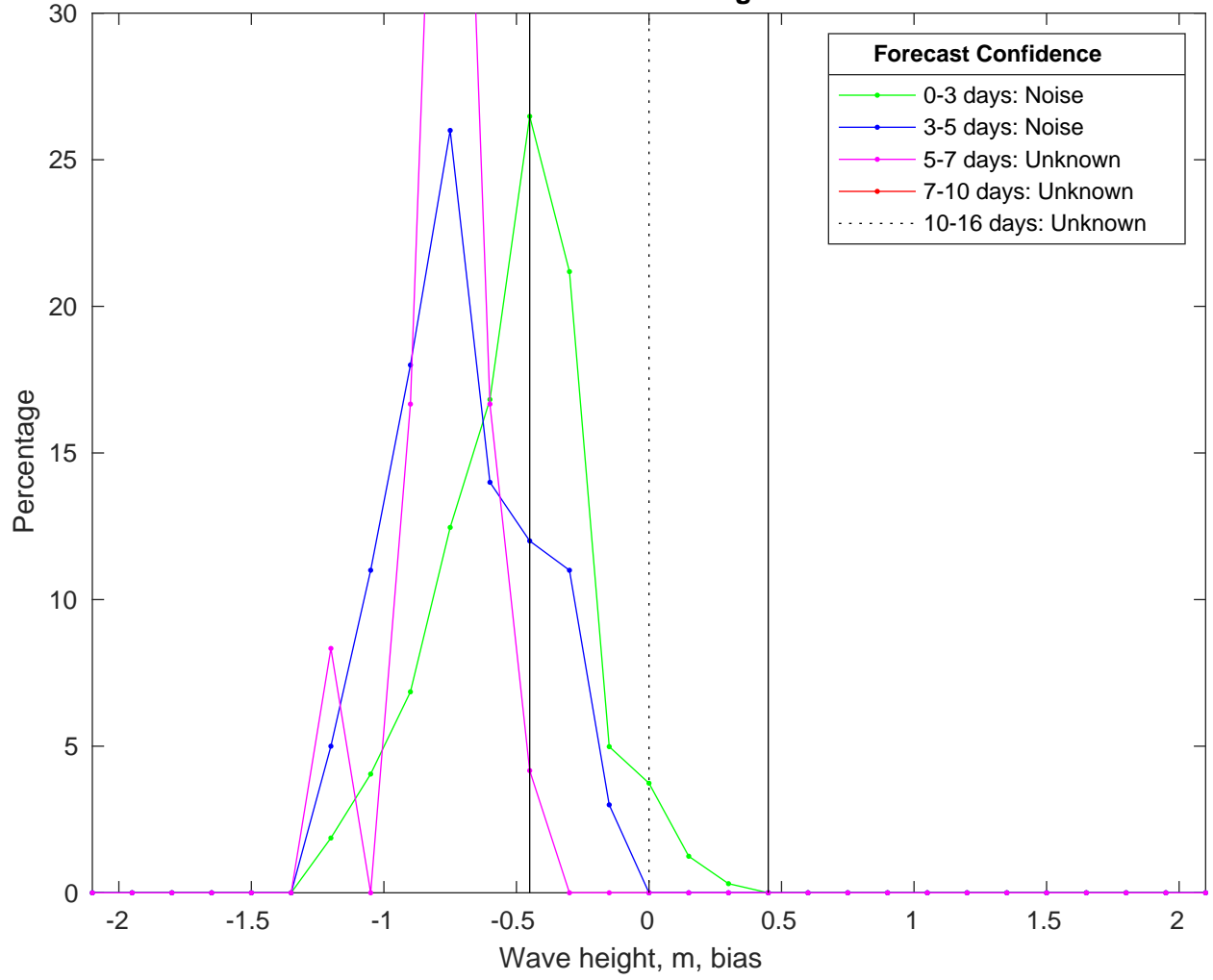
NDBC 51209 vs CMEMSWaves Bias Histogram: 15-Jan-2025
