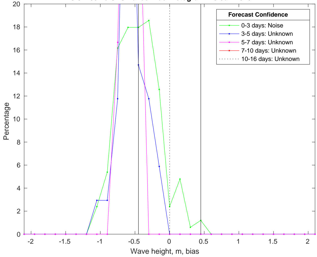
NDBC 51209 vs GFSWaves Bias Histogram: 15-Jan-2025
