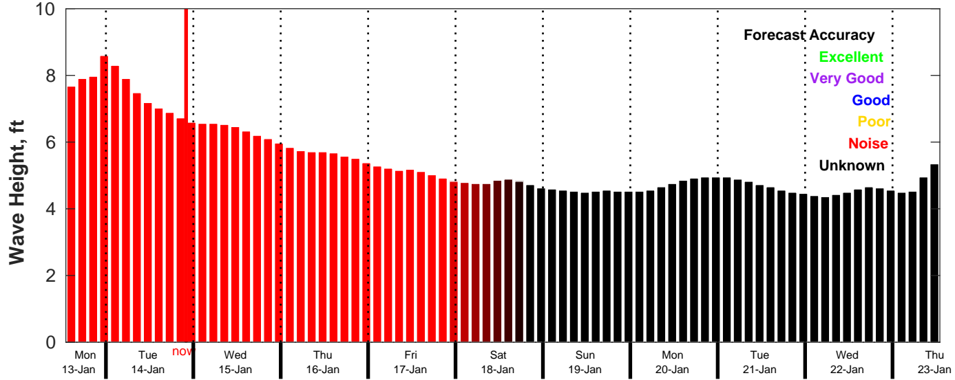
CMEMS Wave Forecast for NDBC 51209 from 13-Jan-2025 13:00:00 to 23-Jan-2025 13:00:00
