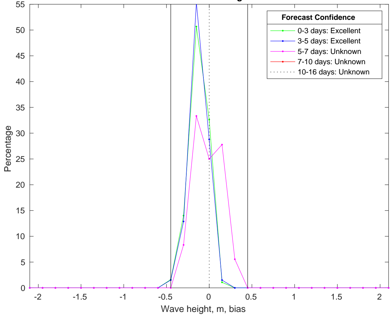
NDBC 52211 vs CMEMSWaves Bias Histogram: 15-Jan-2025
