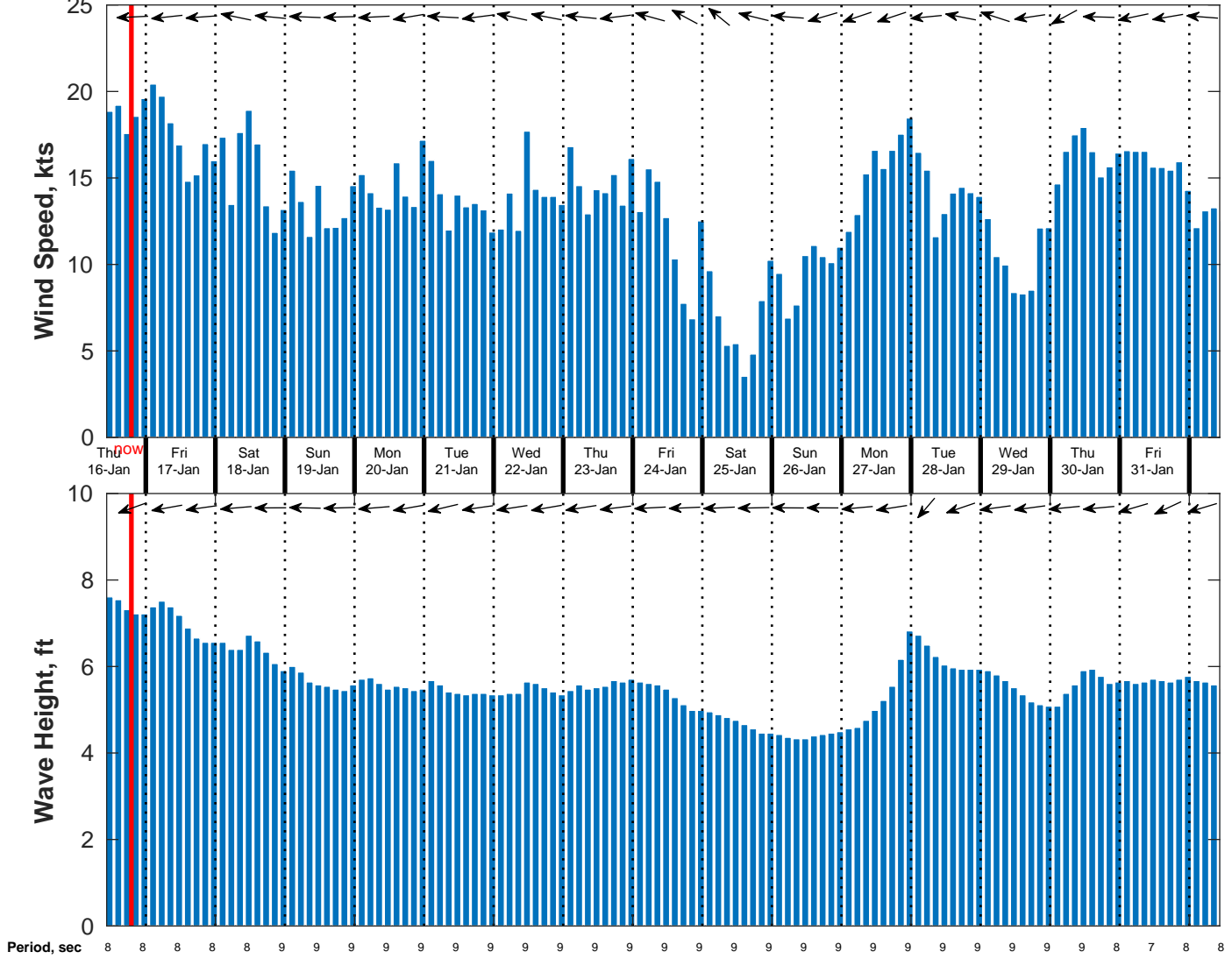
Wind & Wave Forecast for NDBC 52211 from 15-Jan-2025 10:00:00 to 31-Jan-2025 10:00:00
