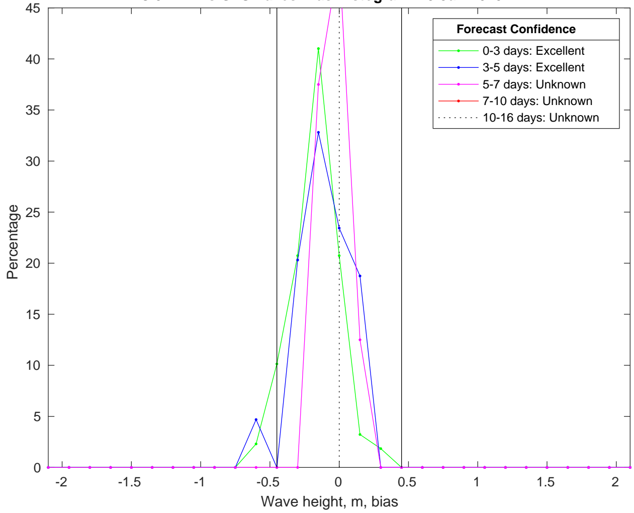
NDBC 52212 vs GFSWaves Bias Histogram: 15-Jan-2025
