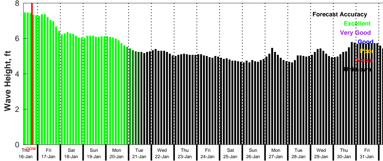
GFS Wave Forecast for NDBC 52212 from 15-Jan-2025 09:00:00 to 31-Jan-2025 09:00:00
