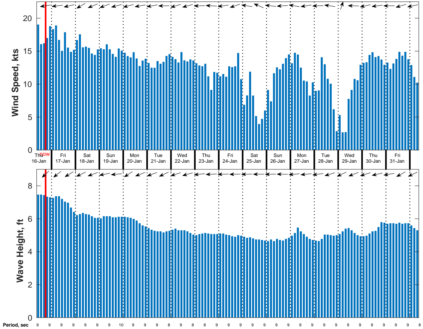
Wind & Wave Forecast for NDBC 52212 from 15-Jan-2025 09:00:00 to 31-Jan-2025 09:00:00
