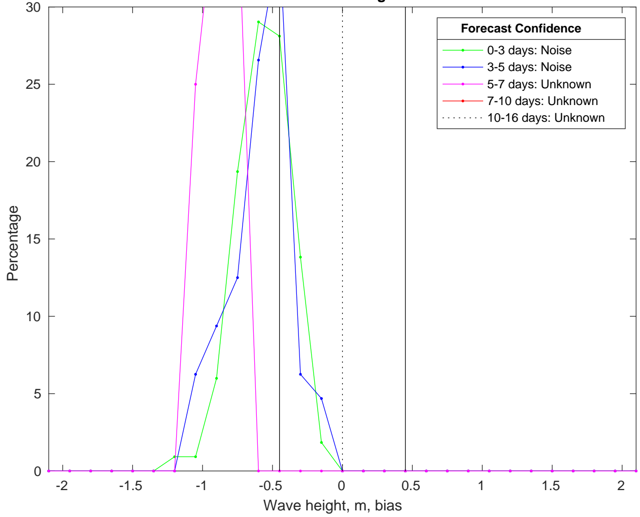
NDBC 52213 vs GFSWaves Bias Histogram: 15-Jan-2025
