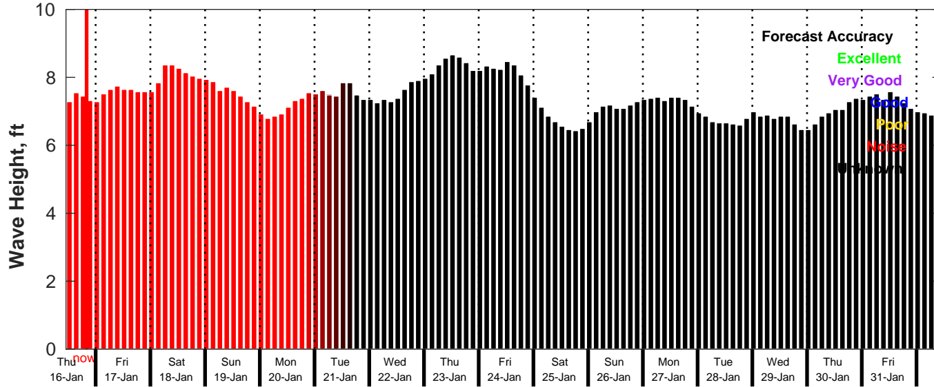
GFS Wave Forecast for NDBC 52213 from 15-Jan-2025 11:00:00 to 31-Jan-2025 11:00:00
