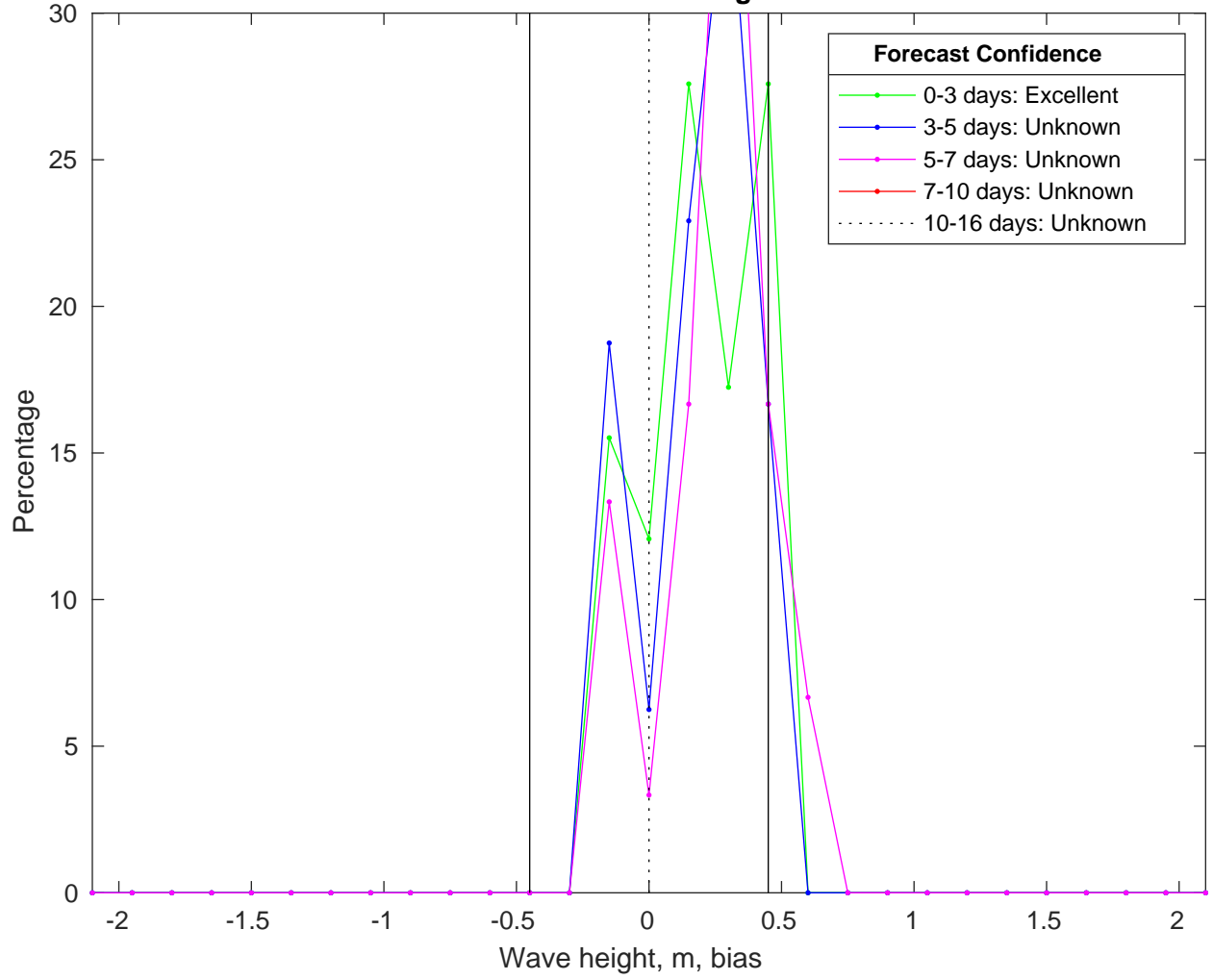
NDBC 62305 vs CMEMSWaves Bias Histogram: 15-Jan-2025
