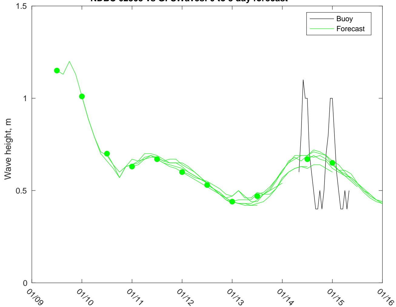
NDBC 62305 vs GFSWaves: 0 to 3 day forecast
