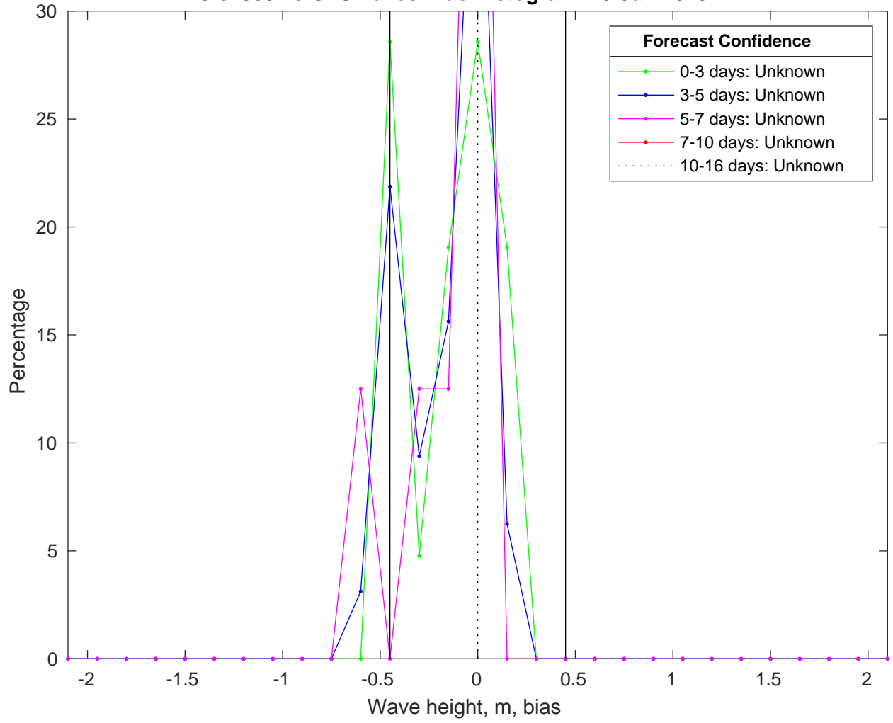
NDBC 62305 vs GFSWaves Bias Histogram: 15-Jan-2025
