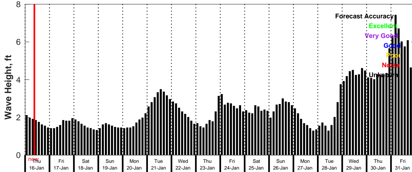
GFS Wave Forecast for NDBC 62305 from 15-Jan-2025 00:00:00 to 31-Jan-2025 00:00:00
