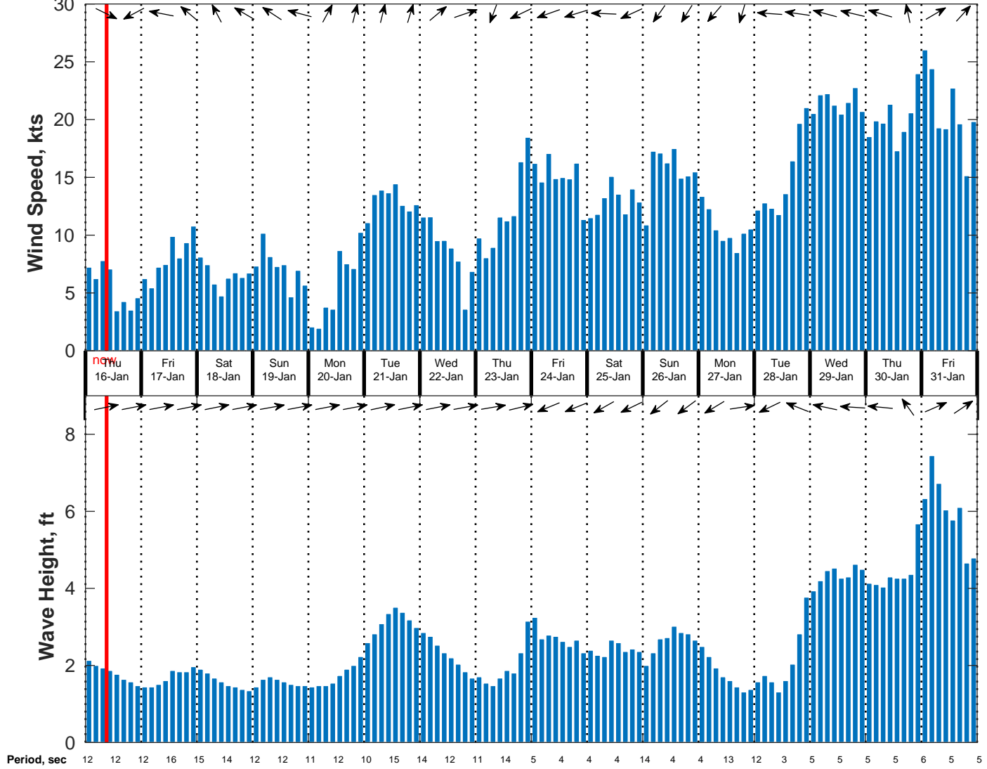
Wind & Wave Forecast for NDBC 62305 from 15-Jan-2025 00:00:00 to 31-Jan-2025 00:00:00
