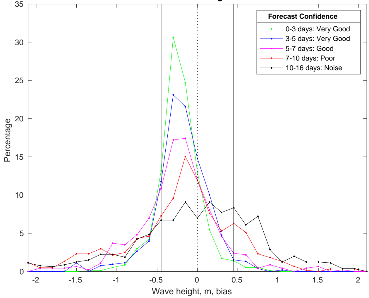
NDBC 41004 vs GFSWaves Bias Histogram: 16-Jan-2025
