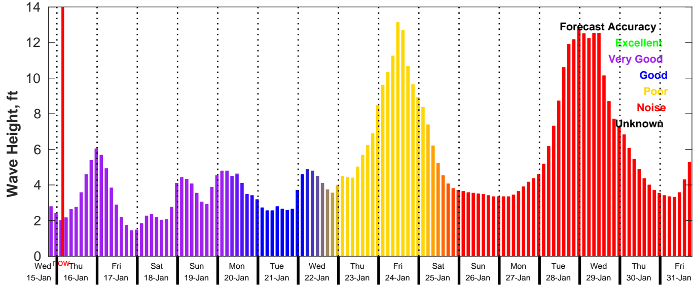
GFS Wave Forecast for NDBC 41004 from 15-Jan-2025 19:00:00 to 31-Jan-2025 19:00:00
