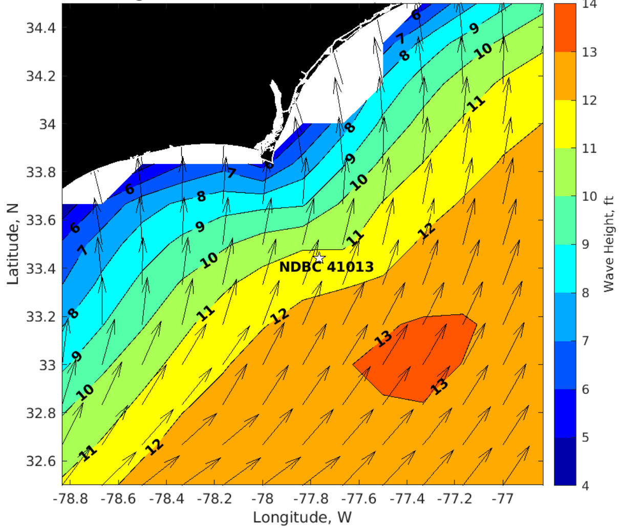
Wave Height (ft) for NDBC 41013 at 12-Dec-2024 00:00:00
