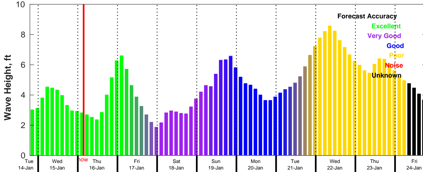
CMEMS Wave Forecast for NDBC 41013 from 14-Jan-2025 19:00:00 to 24-Jan-2025 19:00:00
