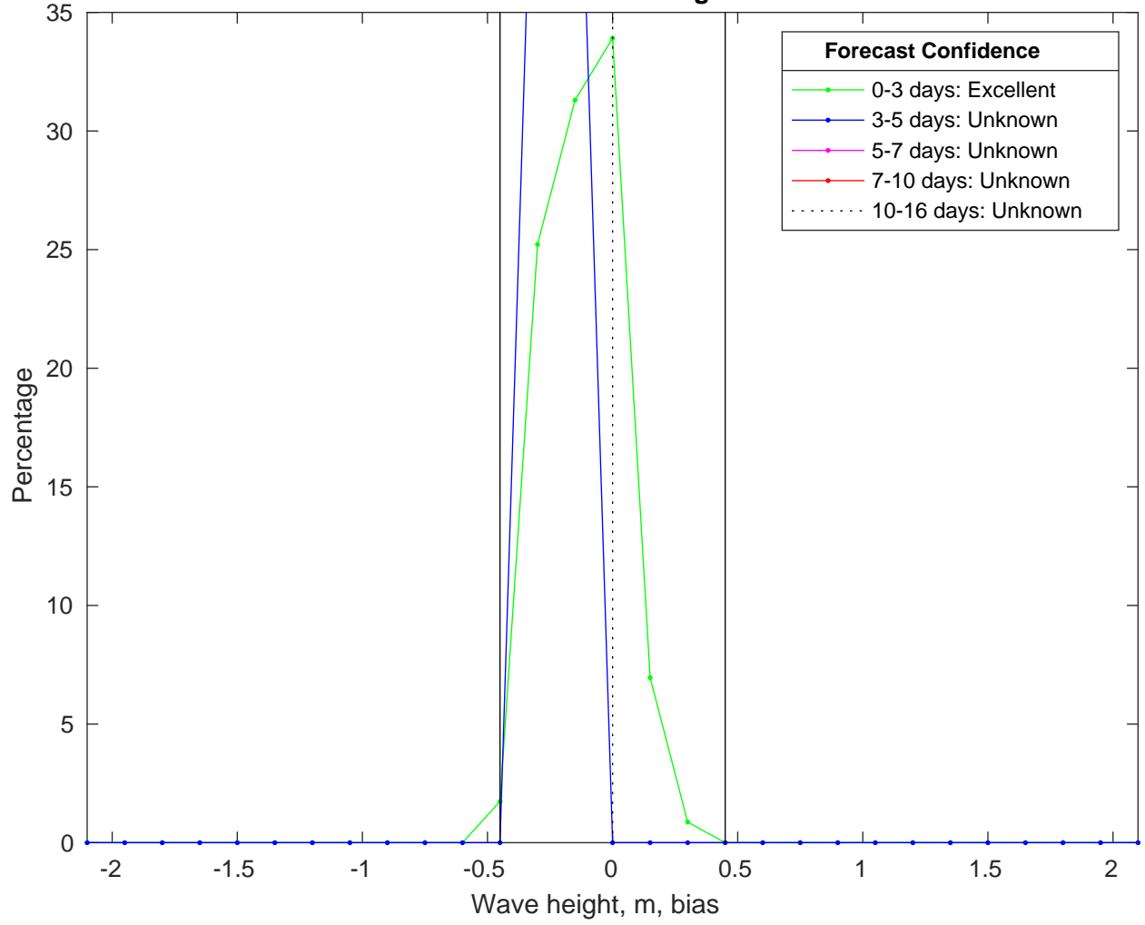
NDBC 41040 vs CMEMSWaves Bias Histogram: 16-Jan-2025
