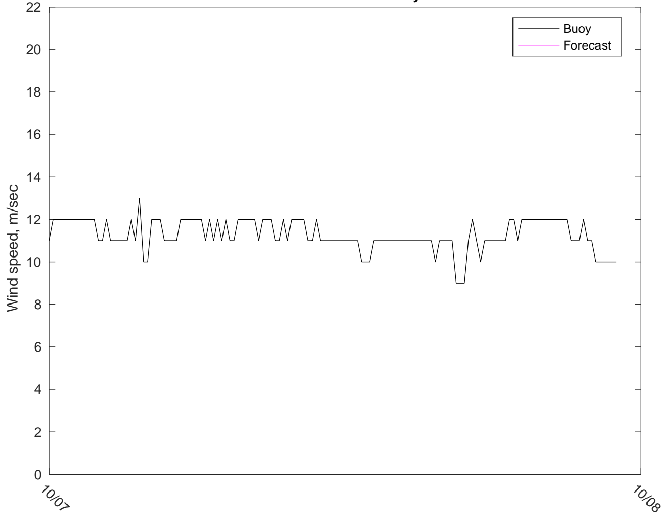
NDBC 42002 vs GFSWinds: 7 to 10 day forecast
