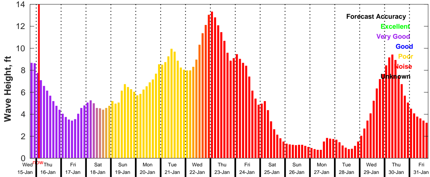
GFS Wave Forecast for NDBC 42019 from 15-Jan-2025 18:00:00 to 31-Jan-2025 18:00:00
