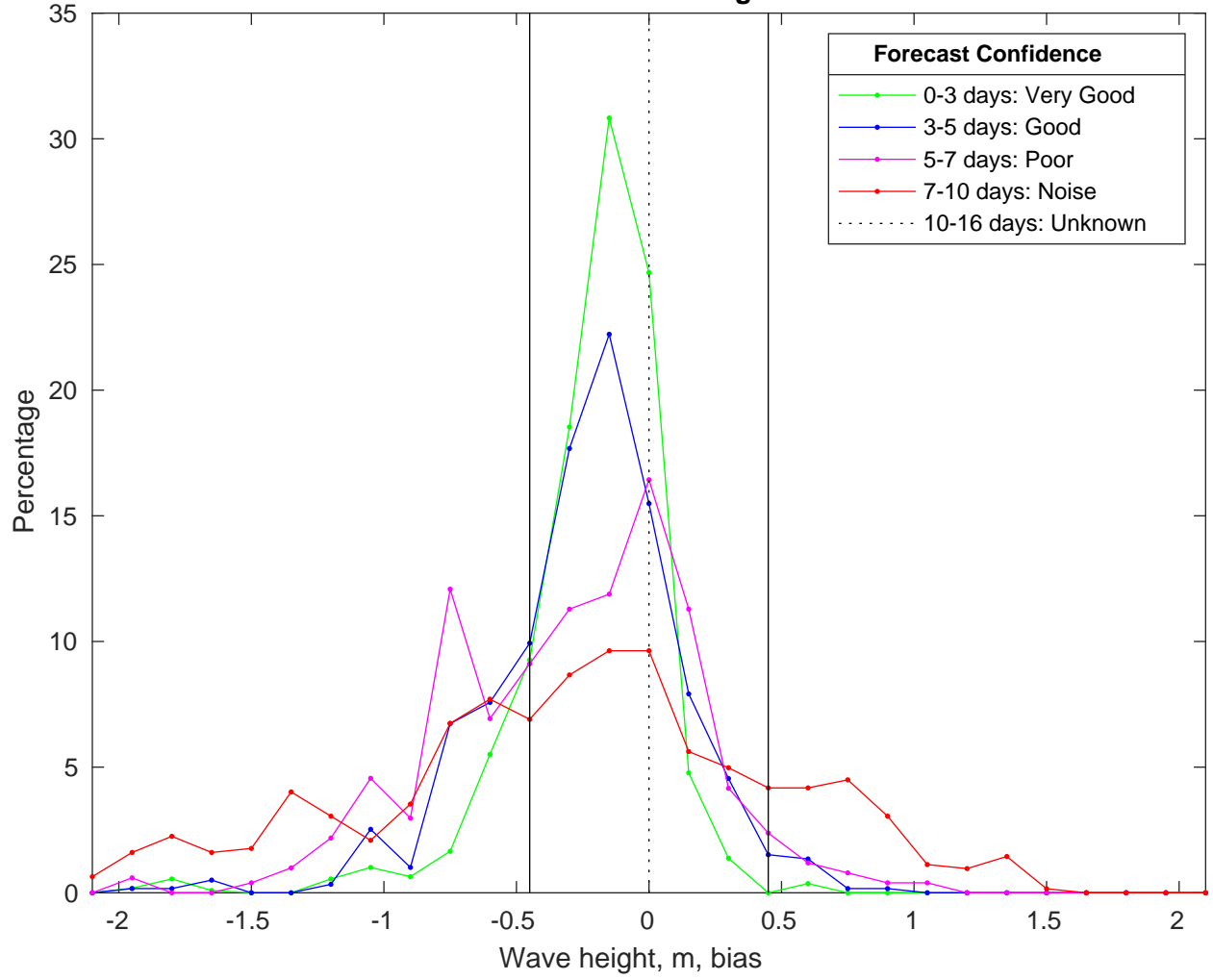
NDBC 42020 vs CMEMSWaves Bias Histogram: 16-Jan-2025
