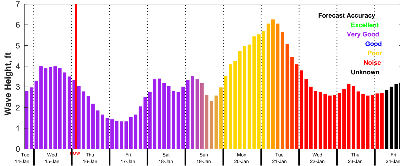
CMEMS Wave Forecast for NDBC 42035 from 14-Jan-2025 18:00:00 to 24-Jan-2025 18:00:00
