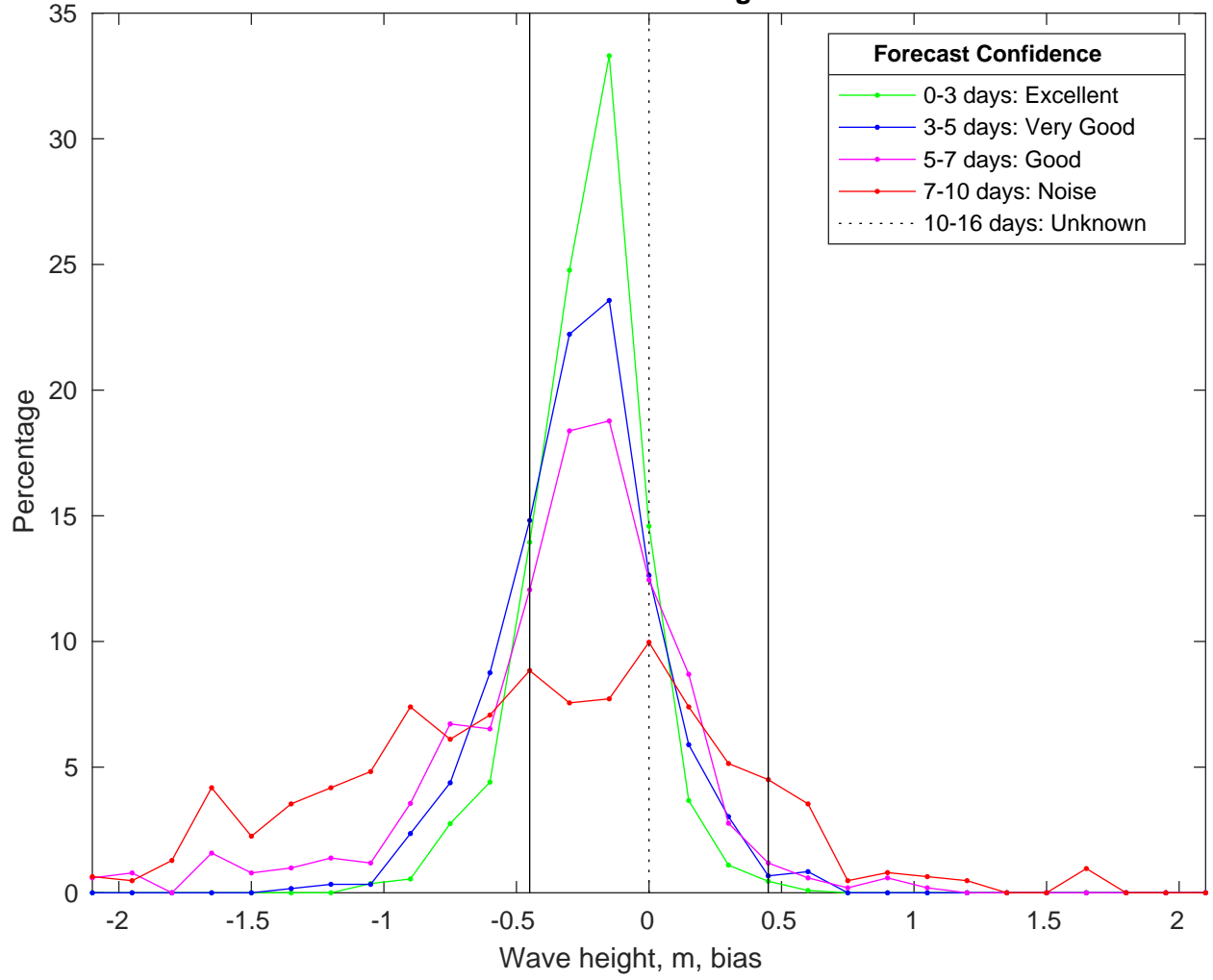
NDBC 42036 vs CMEMSWaves Bias Histogram: 16-Jan-2025
