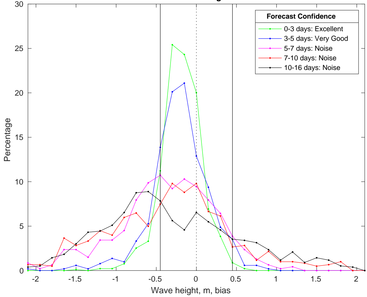
NDBC 42036 vs GFSWaves Bias Histogram: 16-Jan-2025
