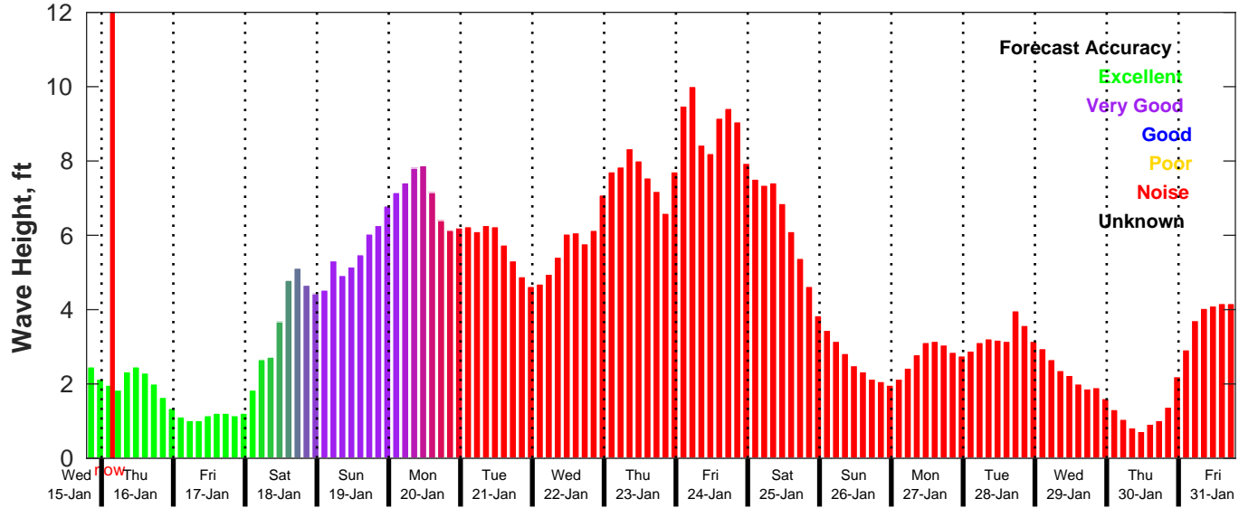
GFS Wave Forecast for NDBC 42036 from 15-Jan-2025 19:00:00 to 31-Jan-2025 19:00:00
