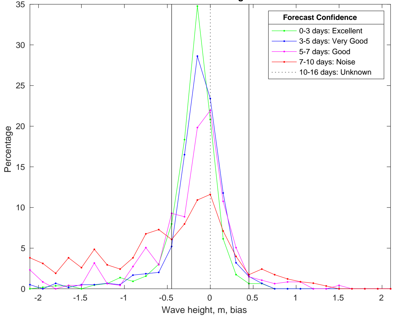
NDBC 42040 vs CMEMSWaves Bias Histogram: 16-Jan-2025
