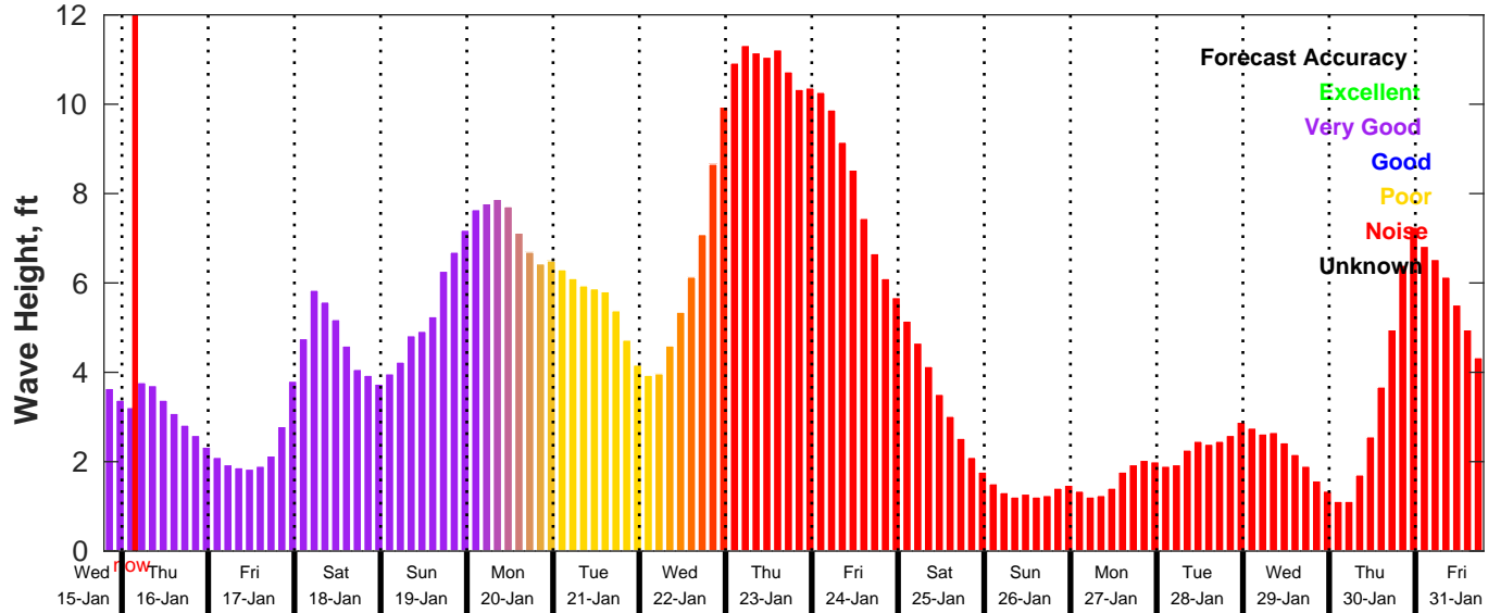
GFS Wave Forecast for NDBC 42040 from 15-Jan-2025 19:00:00 to 31-Jan-2025 19:00:00
