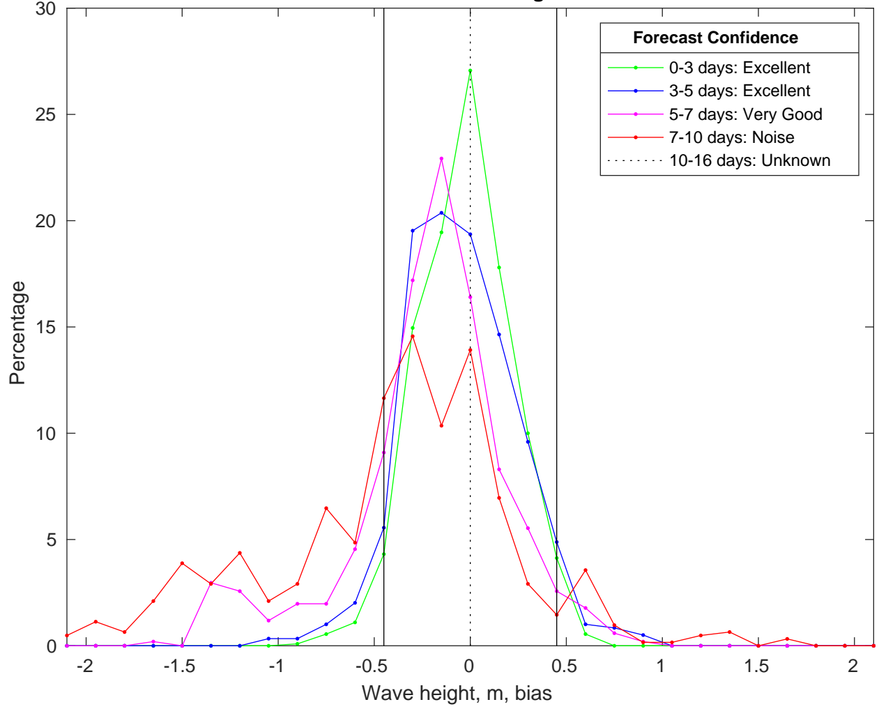
NDBC 42084 vs CMEMSWaves Bias Histogram: 16-Jan-2025
