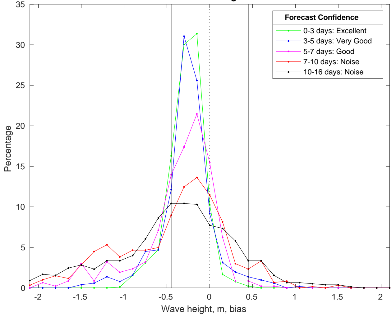
NDBC 42084 vs GFSWaves Bias Histogram: 16-Jan-2025
