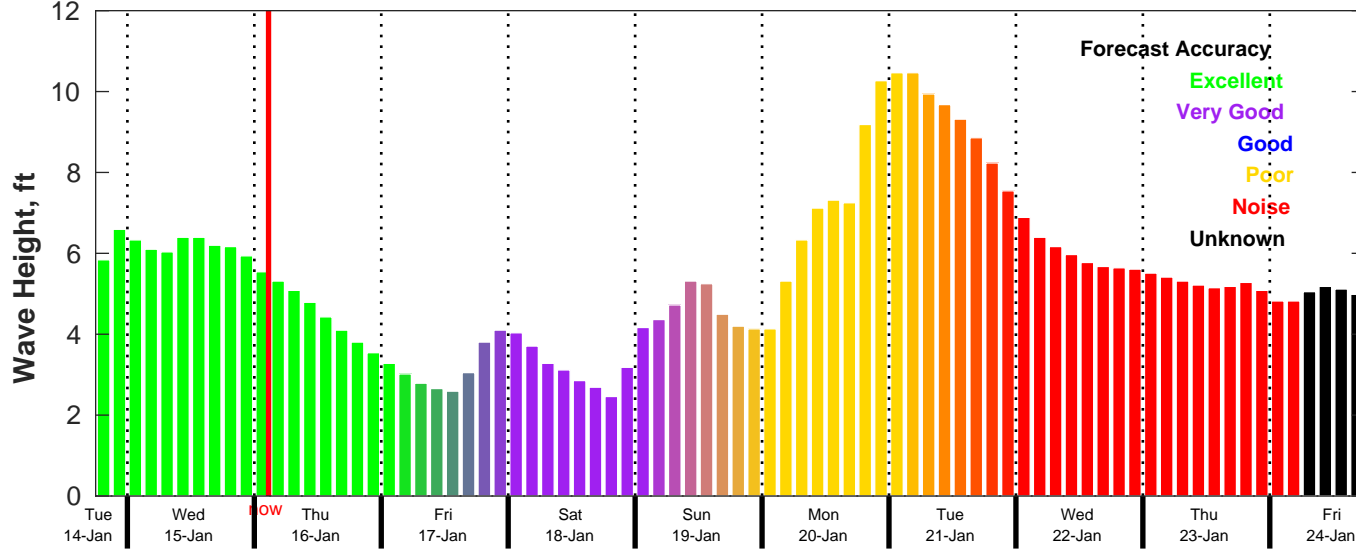
CMEMS Wave Forecast for NDBC 42092 from 14-Jan-2025 18:00:00 to 24-Jan-2025 18:00:00
