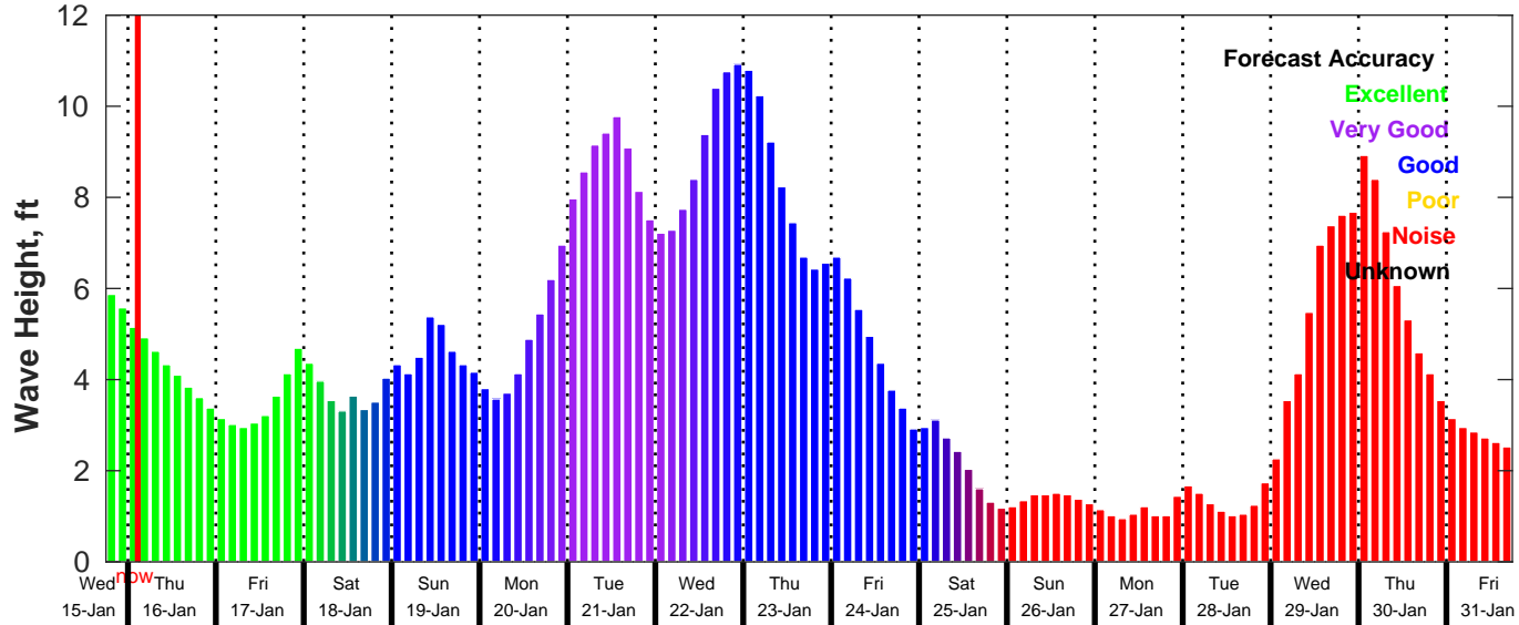
GFS Wave Forecast for NDBC 42092 from 15-Jan-2025 18:00:00 to 31-Jan-2025 18:00:00
