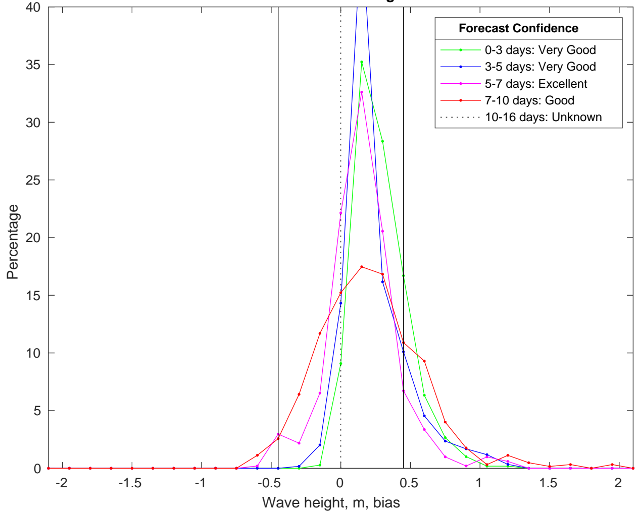
NDBC 44020 vs CMEMSWaves Bias Histogram: 16-Jan-2025
