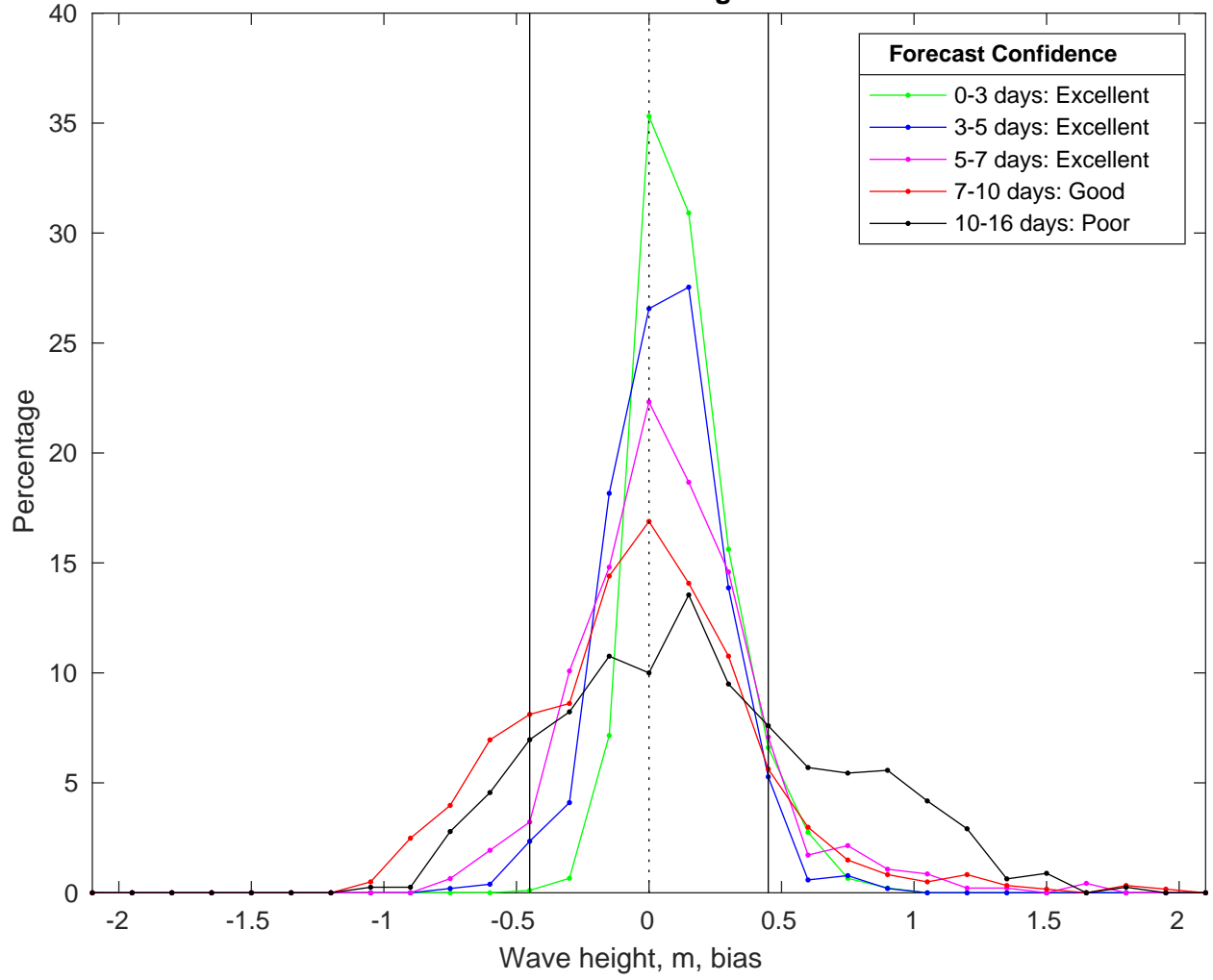
NDBC 44020 vs GFSWaves Bias Histogram: 16-Jan-2025
