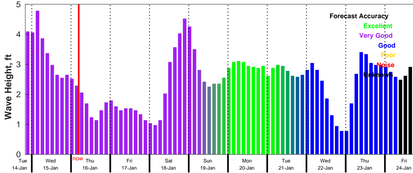
CMEMS Wave Forecast for NDBC 44020 from 14-Jan-2025 20:00:00 to 24-Jan-2025 20:00:00
