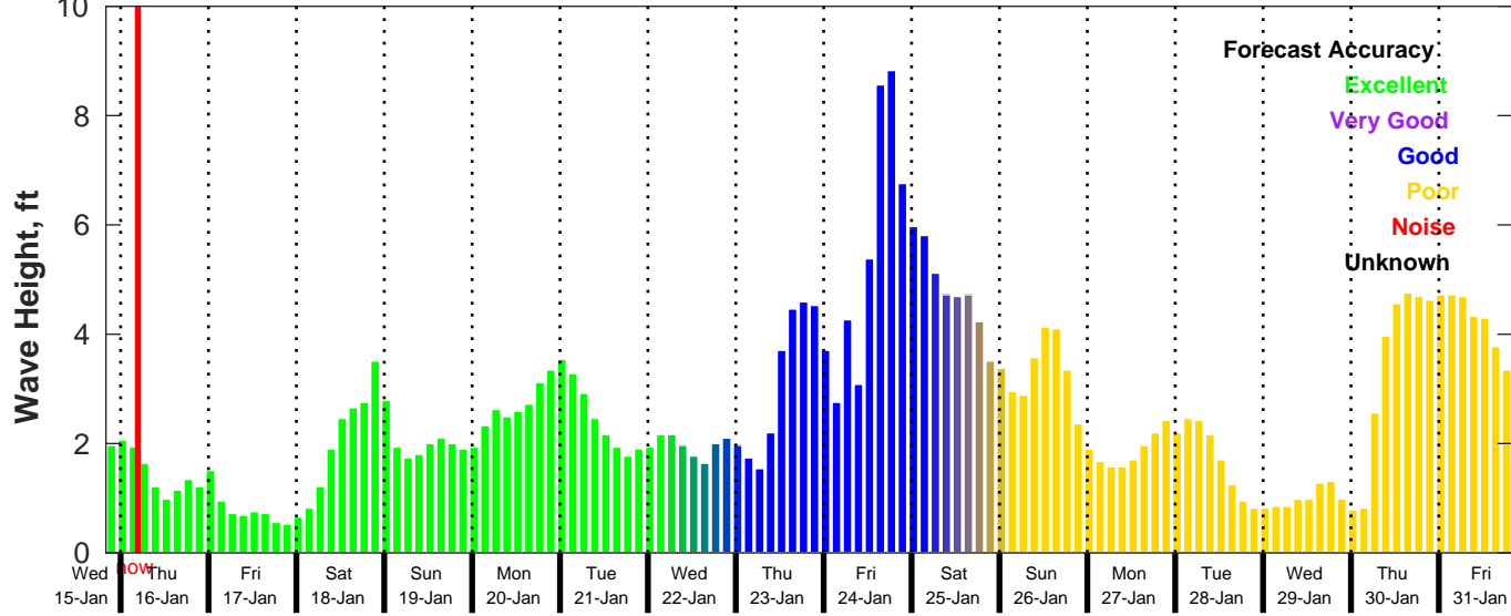
GFS Wave Forecast for NDBC 44020 from 15-Jan-2025 20:00:00 to 31-Jan-2025 20:00:00
