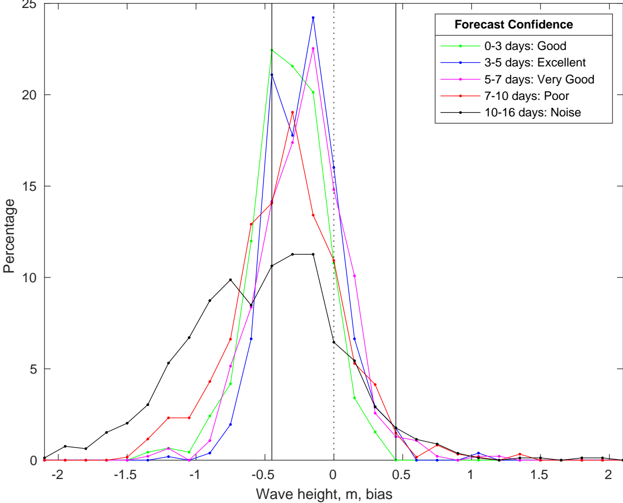
NDBC 46011 vs GFSWaves Bias Histogram: 16-Jan-2025
